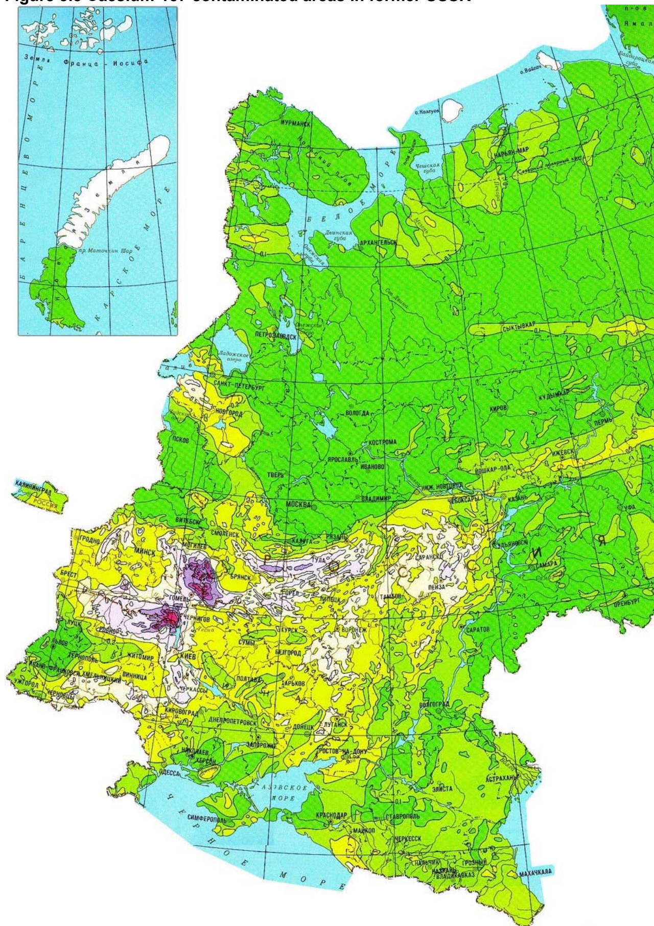
Figure 3.5 Caesium-137 contaminated areas in former USSR
