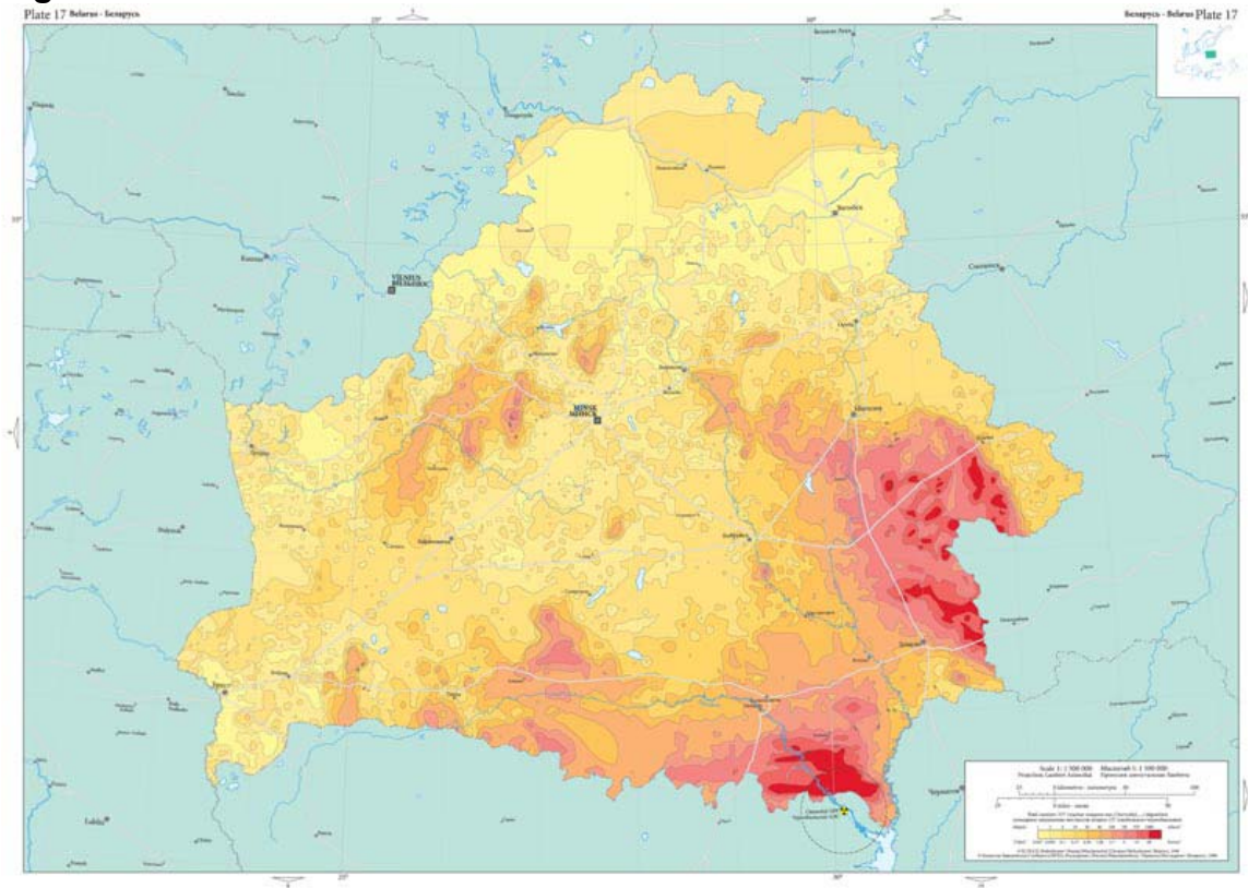
Figure 3.3 Caesium-137 contaminated areas in Belarus
